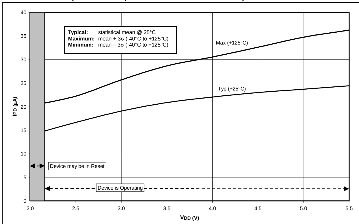
FIGURE 19-17: \Delta I_{PD} BOR vs. V_{DD} , -40°C TO +125°C (SLEEP MODE, BOR ENABLED AT 2.00V-2.16V)
