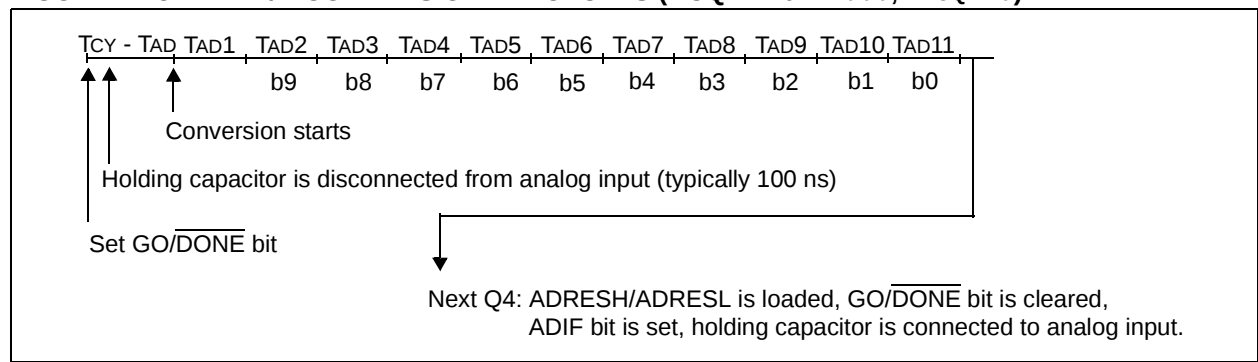
FIGURE 12-3: A/D CONVERSION \text{TAD} CYCLES ( \text{ACQT}<2:0> = 000 , \text{TACQ} = 0 )
