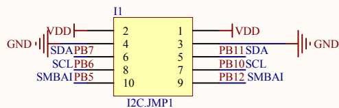
I2C1
