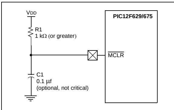
FIGURE 9-5: RECOMMENDED MCLR CIRCUIT
