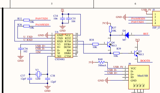
USB接口转串口TTL
