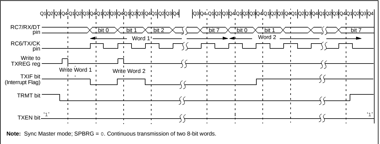
FIGURE 10-9: SYNCHRONOUS TRANSMISSION
