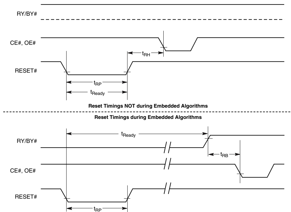
Figure 11.7 Reset Timings
