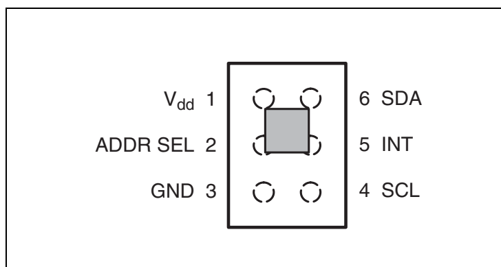
Figure 4: Package FN Dual Flat No-Lead
