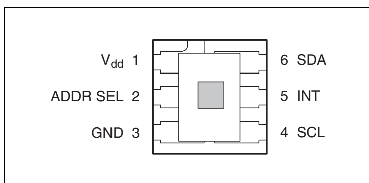
Figure 4: Package FN Dual Flat No-Lead
