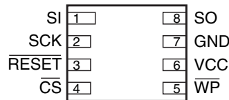
Figure 2-2. SOIC Top View
